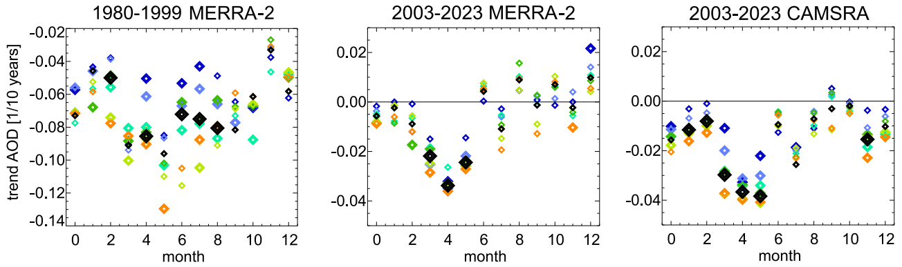
Figure 6. Seasonal variations in trends in monthly mean AOD for selected sectors and the entire Baltic Sea. Colours indicate sectors (see Figure 1), black colour indicates trends in means for the entire Baltic Sea, month=0 indicates trends in annual means, and larger symbols indicate statistically significant trends at a significance level of 0.05. Individual graphs show trends for different reanalyses and periods: MERRA-2 1980–1999 (left), 2003–2023 (middle) and CAMS 2003–2023 (right).
