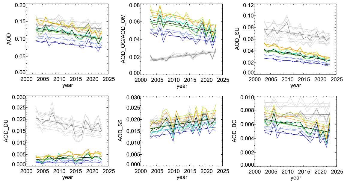
Figure 5. Temporal variability of annual spatial means of AOD and speciated AODs from CAMSRA for the entire Baltic Sea (black) and the sectors (colours indicate sectors as in Figure 1). Straight lines show the corresponding trends for the period 2003–2023. The corresponding time series of total AOD and speciated AODs from MERRA-2 (from Figure 4) are plotted in grey for comparison.
