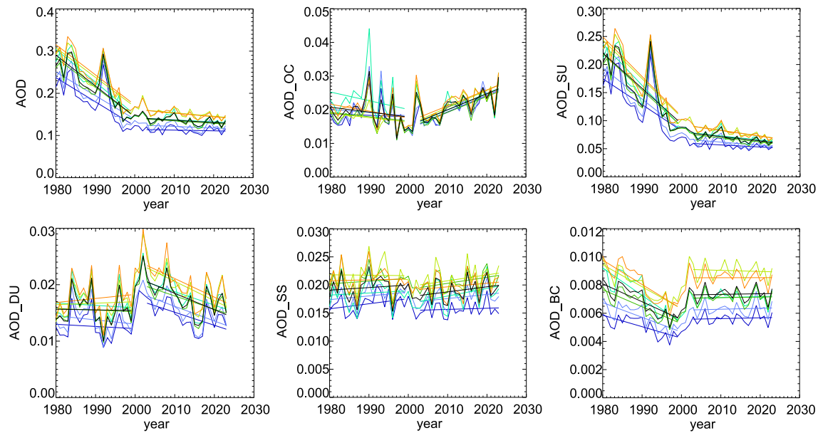
Figure 4. Temporal variability of annual spatial means of AOD and speciated AODs from MERRA-2 for the entire Baltic Sea (black) and the sectors (colours indicate sectors as in Figure 1). Straight lines represent the corresponding trends for the periods 1980–1999 and 2003–2023.
