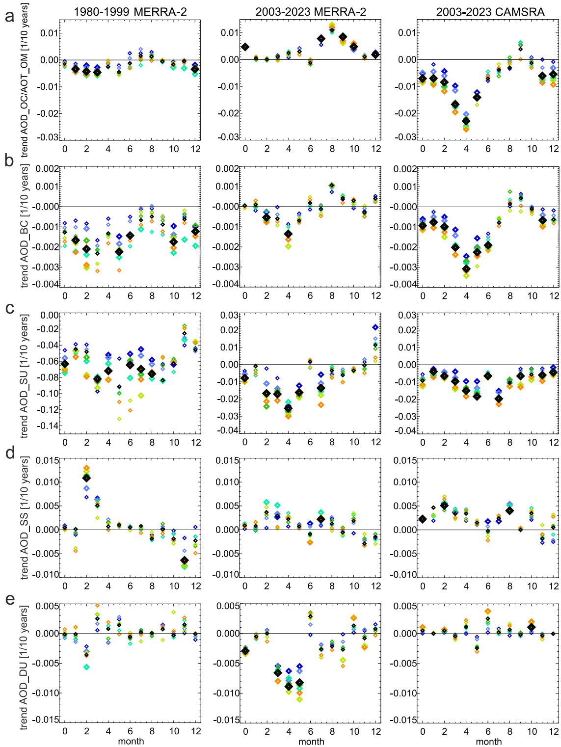
Figure 7. Seasonal changes in trends in monthly mean speciated AOD: a) AOD_OC, b) AOD_BC, c) AOD_SU, d) AOD_SS, and e) AOD_DU, for selected sectors and the entire Baltic Sea. Colours indicate sectors (see Figure 1), black indicates trends in the means for the entire Baltic Sea, month=0 indicates trends in annual means, and larger symbols indicate trends statistically significant at a significance level of 0.05. Columns show trends for different reanalyses and periods: MERRA-2 1980–1999 (left), 2003–2023 (middle) and CAMS 2003–2023 (right).
