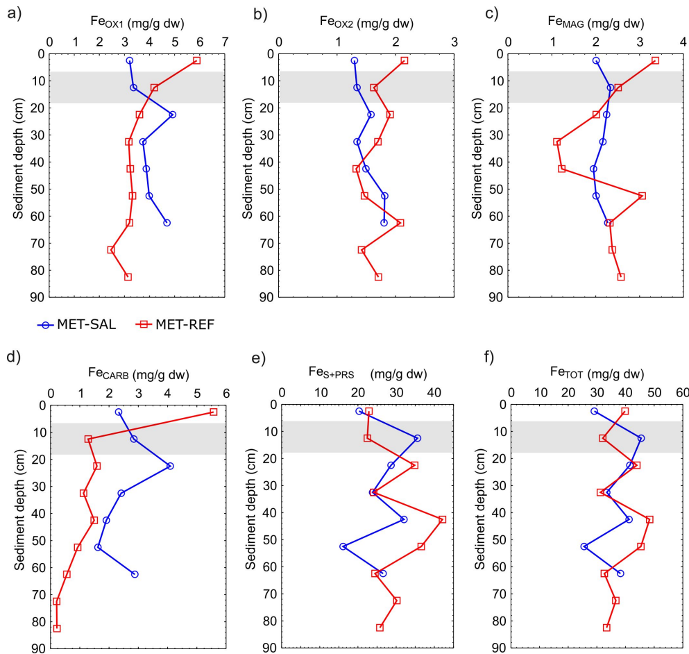
Figure 5. Concentration of iron in labile oxyhydroxides ( Fe_{OX1} ) (a), iron in crystalline oxyhydroxides ( Fe_{OX2} ) (b), iron in magnetite ( Fe_{MAG} ) (c), iron in carbonates ( Fe_{CARB} ) (d), iron in sulfides and poorly reactive silicate sheets ( Fe_{S+PRS} ) (e), and total iron ( Fe_{TOT} ) (f) in sediments of the pockmark MET1-SAL and reference station MET1-REF. Sediments for mineralogical analyses were collected at the depth denoted by gray bars.
