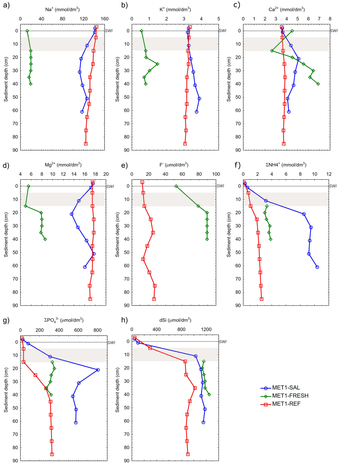
Figure 3. Concentrations of major cations ( \text{Na}^+ – sodium, \text{K}^+ – potassium, \text{Ca}^{2+} – calcium, \text{Mg}^{2+} – magnesium) (a–d), fluoride ( \text{F}^- ) (e), ammonia ( \Sigma\text{NH}_4^+ ) (f), phosphate ( \Sigma\text{PO}_4^{3-} ) (g) and silicate (dSi) (h) in bottom and pore water at three research stations. SWI stands for sediment-water interface. Sediments for mineralogical analyses were collected at the depth denoted by grey bars.
