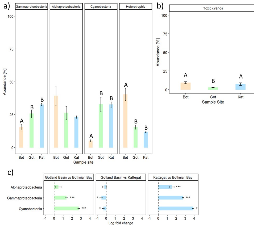
Figure 4. Relative abundances of bacterial taxa at sites. Taxa grouped by photosynthetic potential (a), percentage of cyanobacteria which are potentially toxic (b), taxa which differed significantly between sites as identified by ANCOM-BC analysis (c). Data are means and standard errors. Different letters indicate significant differences ( P < 0.05 ) determined by Tukey's test.
