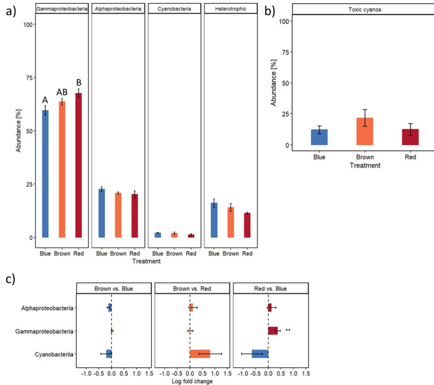
Figure 6. Relative abundances of bacterial taxa for samples from the Bothnian Bay after light incubation. Taxa grouped by photosynthetic potential (a), percentage of cyanobacteria which are potentially toxic (b), taxa which differed significantly after incubation as identified by ANCOM-BC analysis (c). Data are means and standard errors. Different letters indicate significant differences ( P < 0.05 ) determined by Tukey's test.
