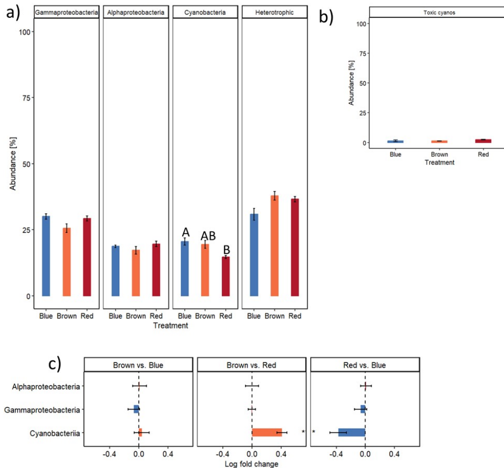
Figure 8. Relative abundances of bacterial taxa for samples from the Gotland Basin after light incubation. Taxa grouped by photosynthetic potential (a), percentage of cyanobacteria which are potentially toxic (b), taxa which differed significantly after incubation as identified by ANCOM-BC analysis (c). Data are means and standard errors. Different letters indicate significant differences ( P < 0.05 ) determined by Tukey's test.
