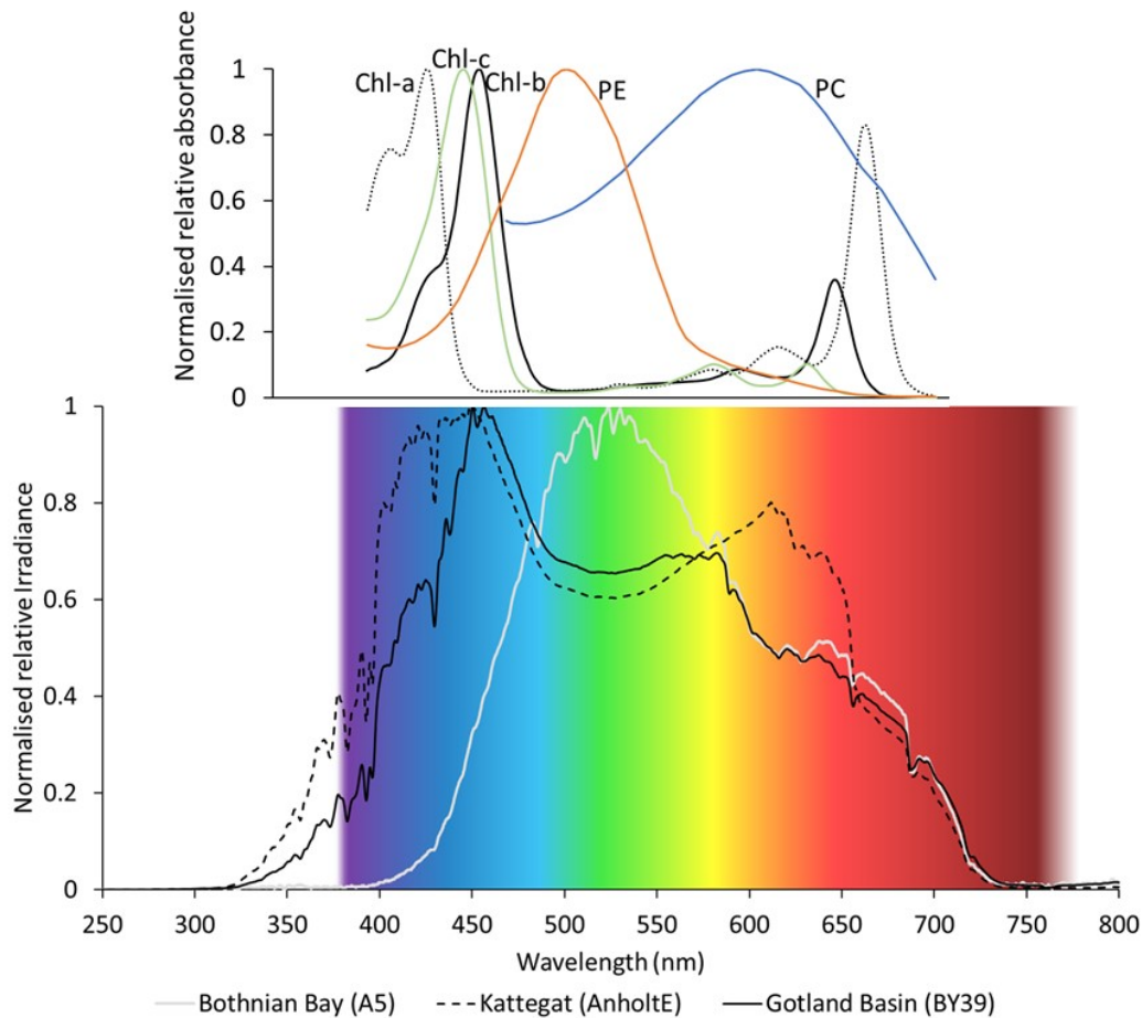
Figure 2. Relative irradiance of light wavelengths at a 2 m depth normalised to maximum irradiance. Absorbance spectra of key algal chlorophylls and pigments from the PhotochemCAD database (Taniguchi and Lindsey, 2023).
